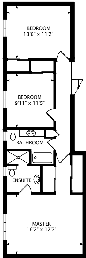
SECOND FLOOR 873 SQUARE FEET
